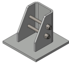
Weld Down Flange
