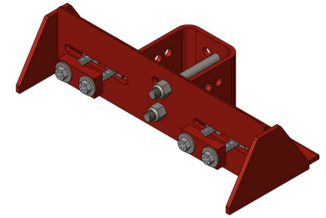
Concrete Rebar Clamp
