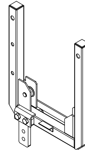
STIRRUP FRAME ASSY:SHORT BB-004R WEIGHT: 13.5 LB
