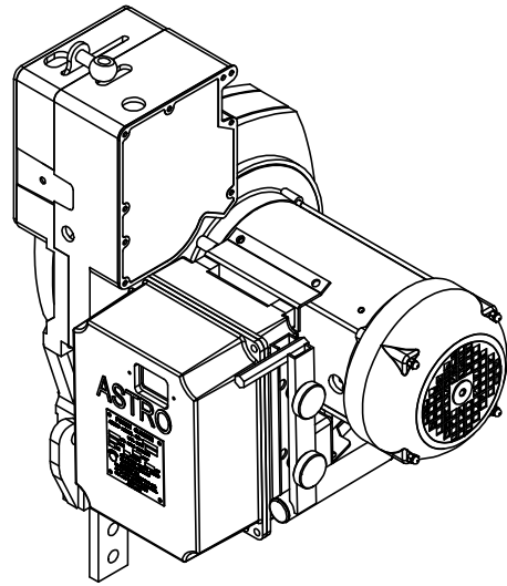
ASTRO B:1PH 220V/60HZ:1.5HP 90.982-1500R WEIGHT: 136 LB
