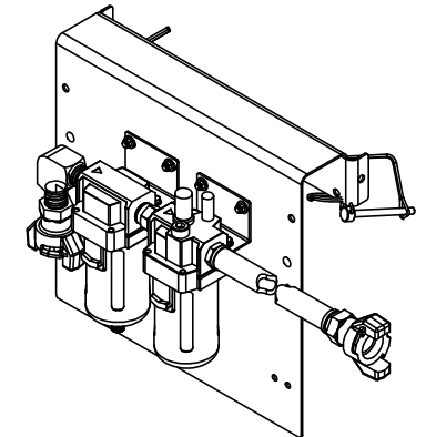
FILTER/LUBRICATR ASSY:PC1/SC30 8-0108R (706126-1) WEIGHT: 7 LB
