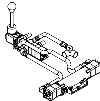
REMOTE CONTROL ASSY:AIR: 9-61-XR WEIGHT: -- LB
