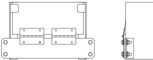
Bottom Arc Guard 700947-1
