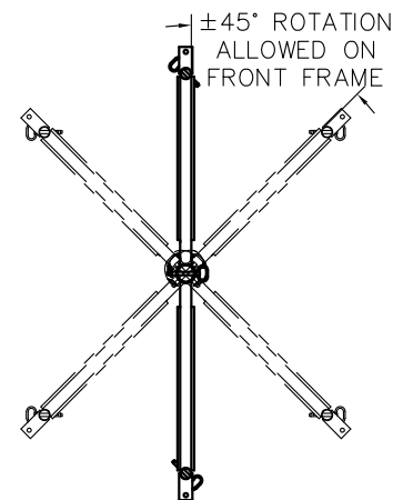
COUNTERWEIGHT TABLE
