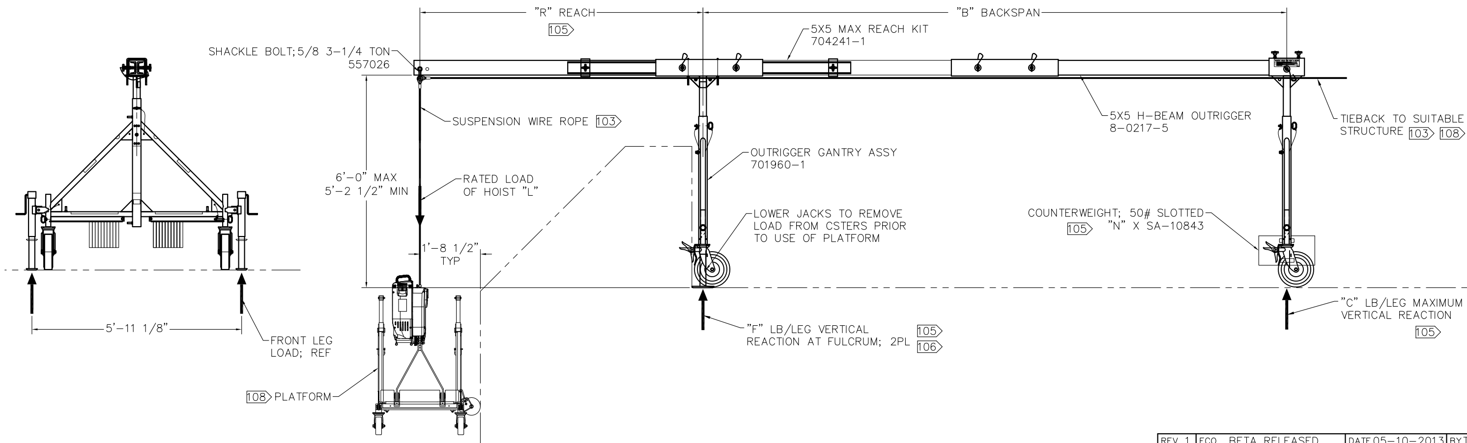
SPIDER ROLLING GANTRY WITH 5X5 OUTRIGGER WITH MAX REACH KIT
